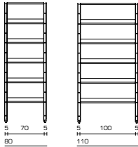
PIANTANA A PARETE UPRIGHT WITH WALL FIXING STANDER FÜR WANDMONTAGE MONTANT À FIXATION MURALE MONTANTE A PARED
